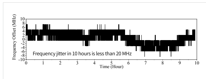
Wavelength Stability
